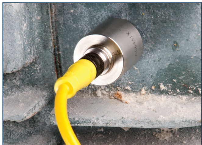
The triaxial accelerometer collects data at the measurement location from a vertical, horizontal, and axial directions simultaneously.
